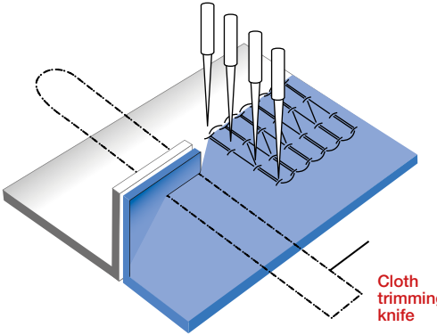
MF-3620L200 subclass is suited to light weight materials and has cloth trimmer on both sides.
